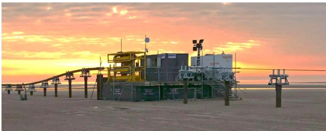
Plate 3.6: Example roller boxes and intermediate pulling platform installation (image courtesy of Boskalis)
